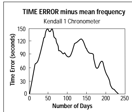
Figure B4. A time error plot after subtracting a calibrated frequency offset from the numbers over the first 230 days — the time it was housed in the first gallery. As compared to Figure B1, notice that this calibration reduces the peak-to-peak error by about a factor of 150. Notice also the general parabolic shape to the curve — indicative of a negative frequency drift.
